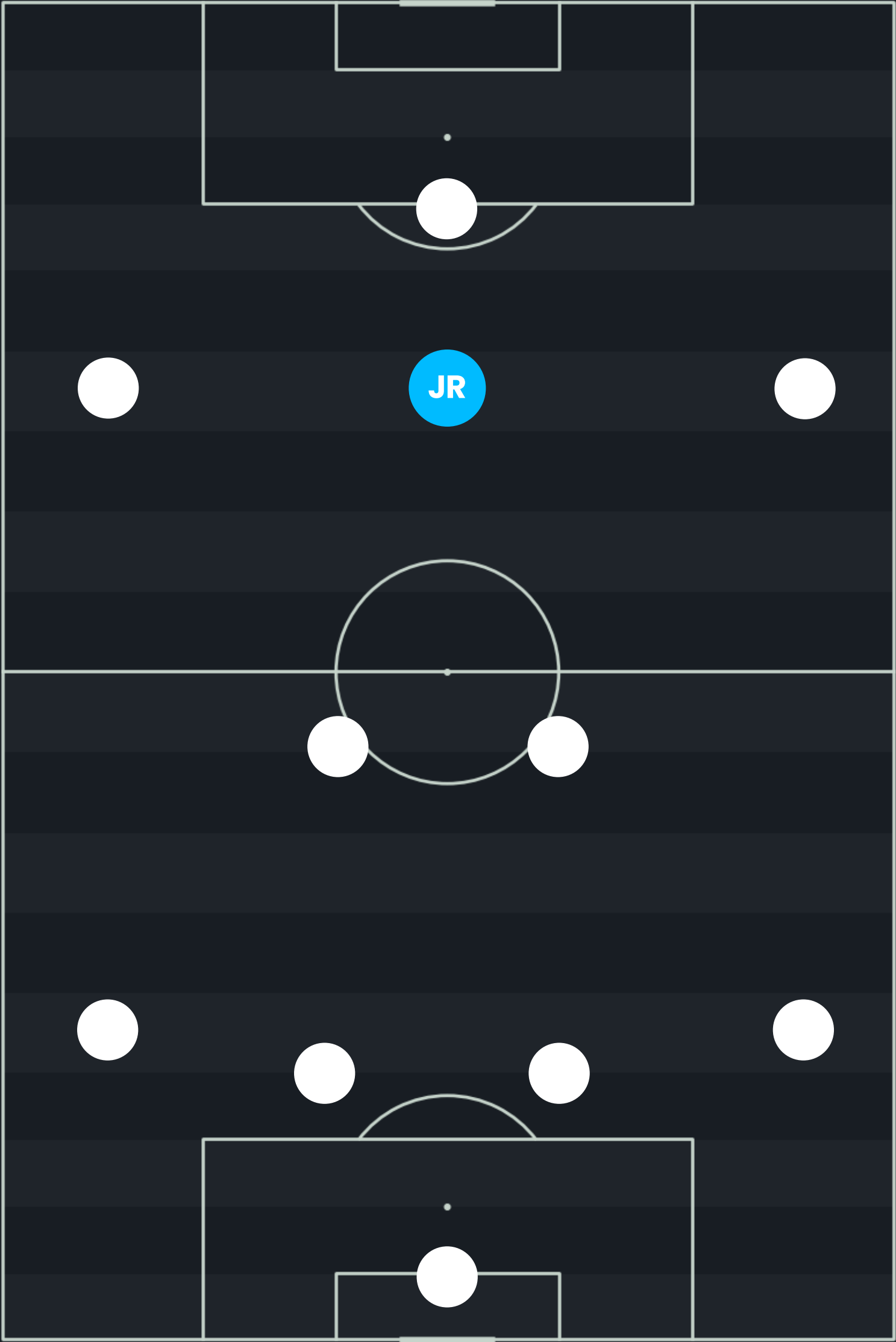
4-2-3-1 (42%)
