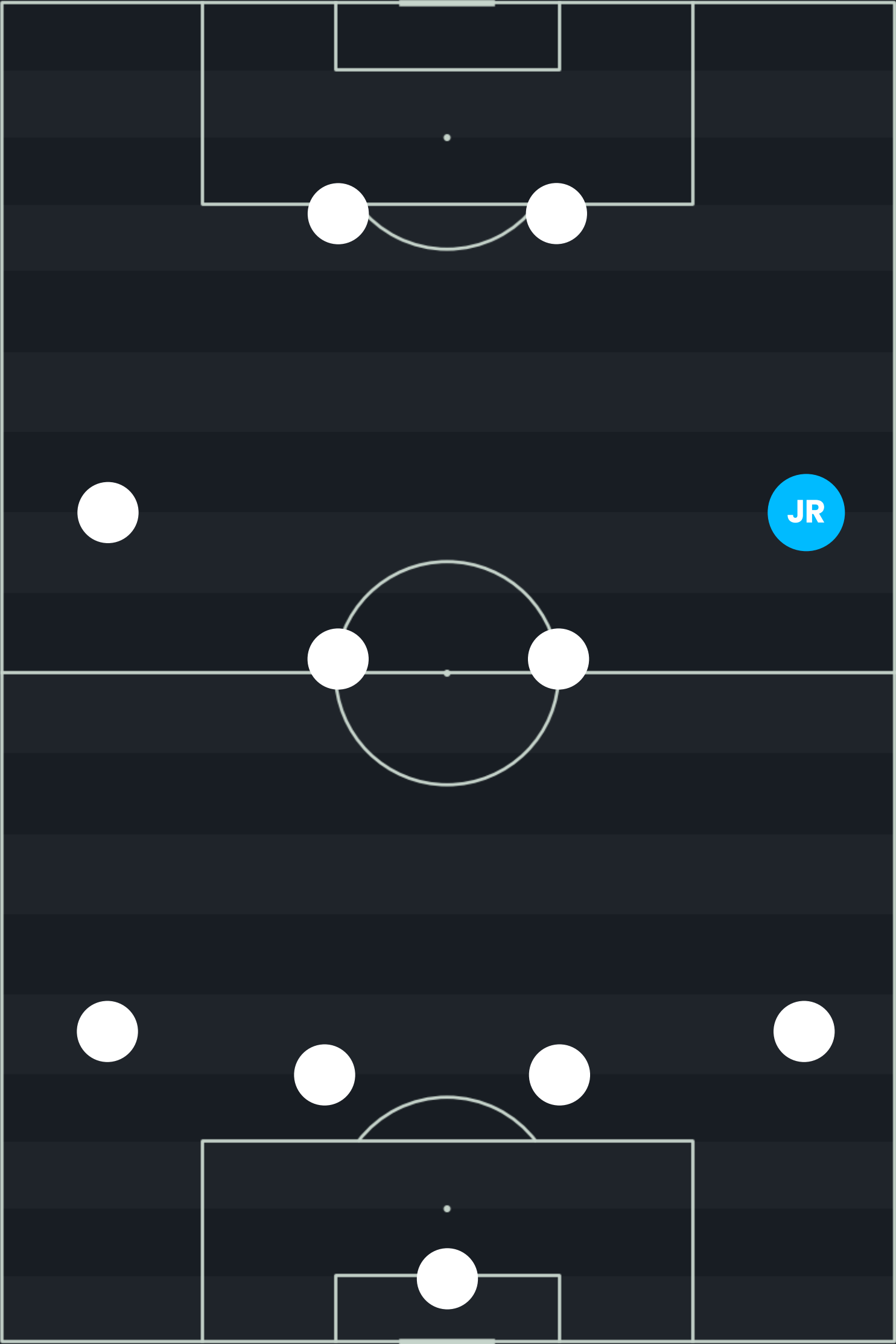
4-4-2 (8%)
