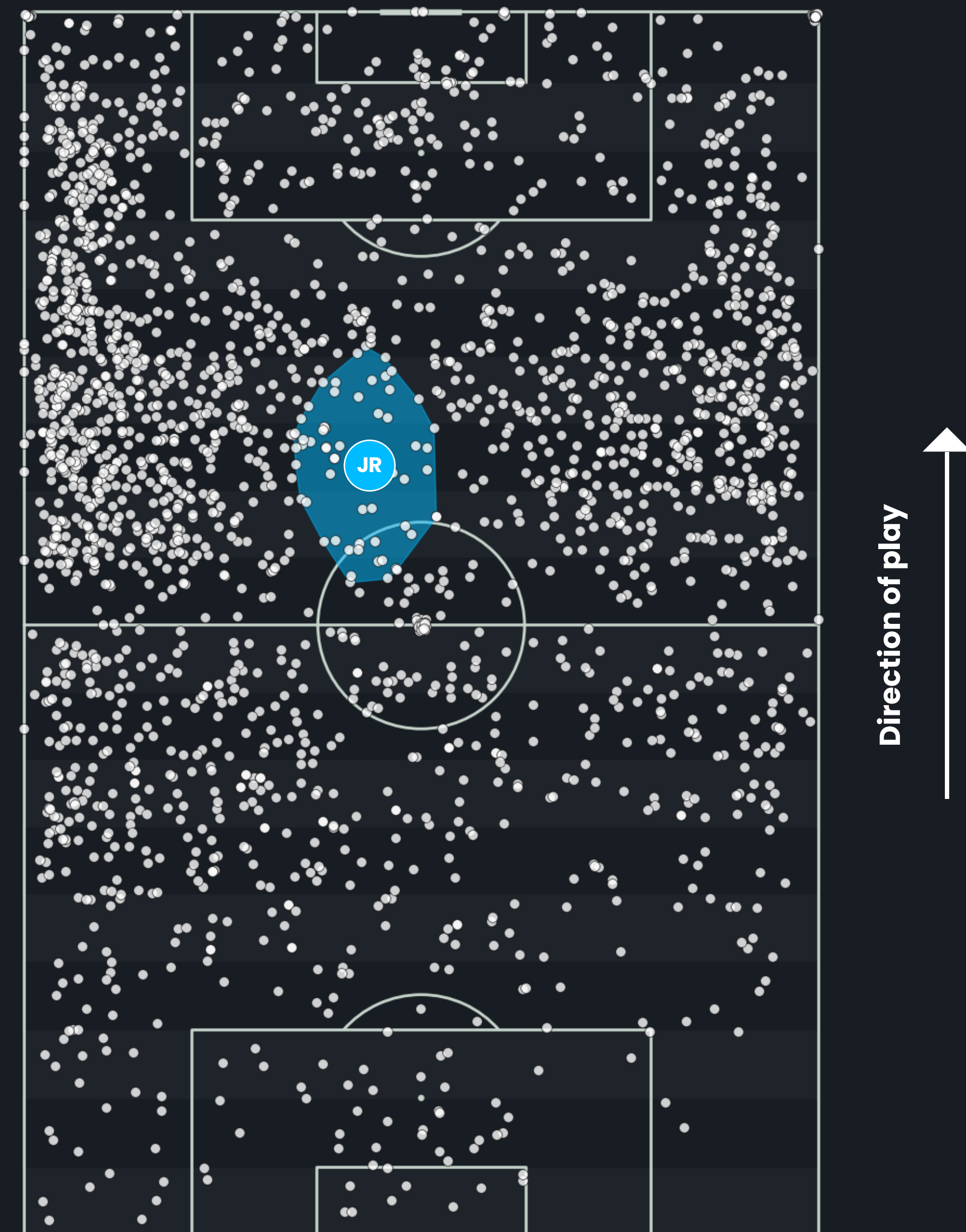
2024–25 Touch Map
