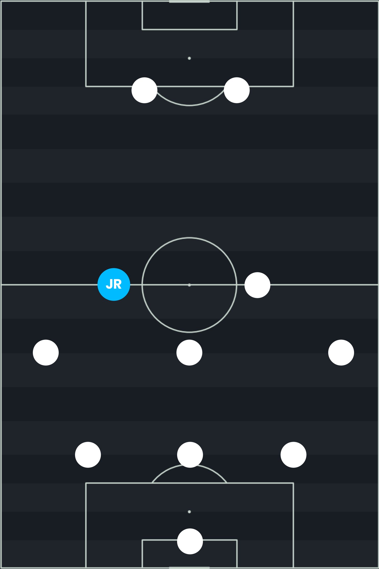
3-5-2 (11%)
